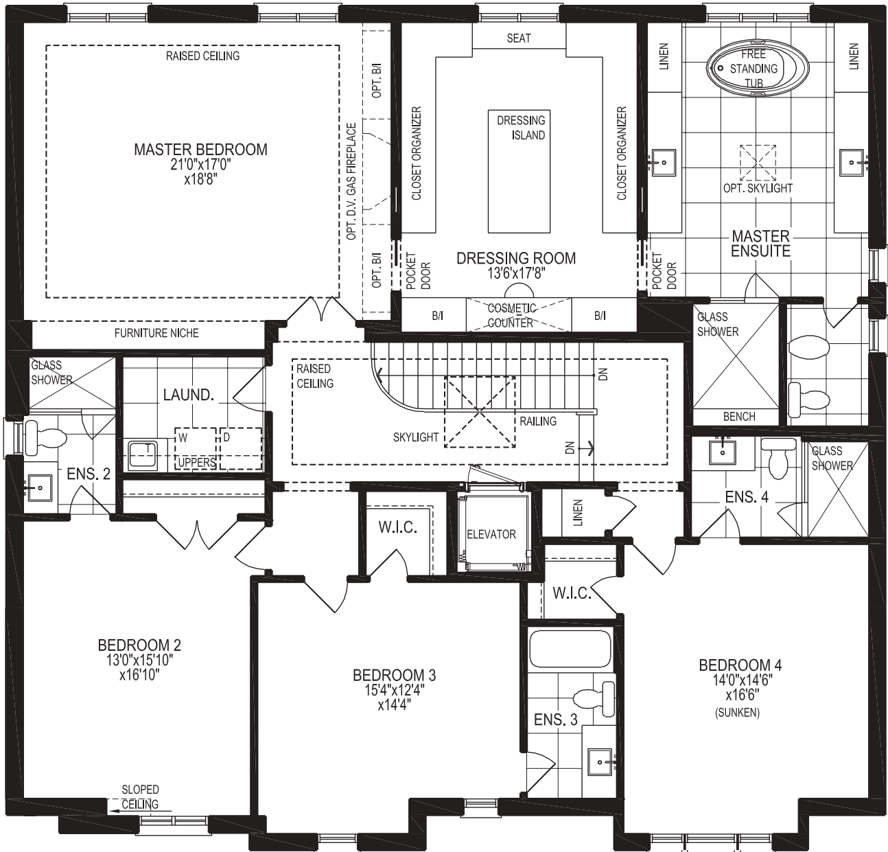
Elevation A SECOND FLOOR
