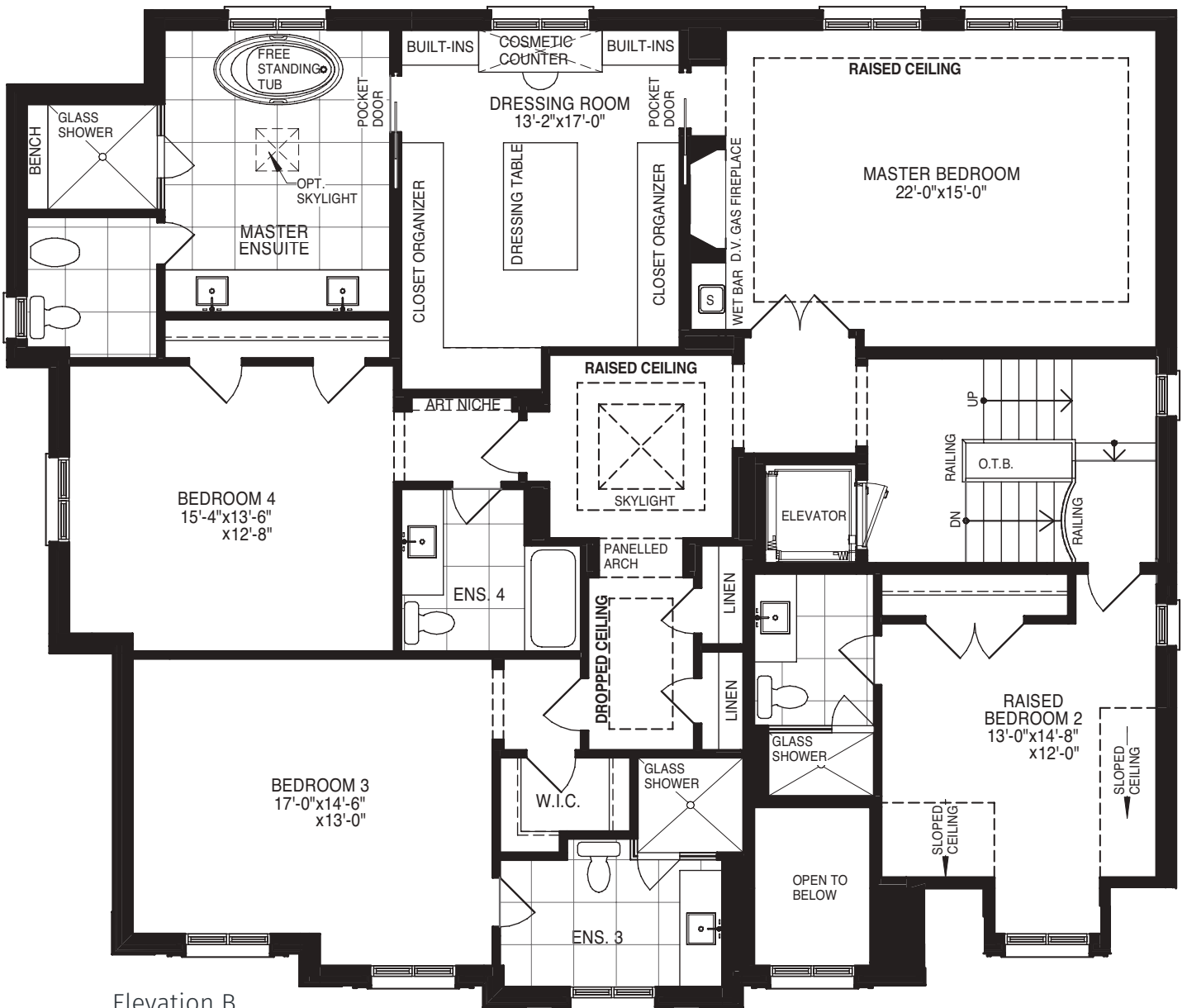
Elevation B SECOND FLOOR
