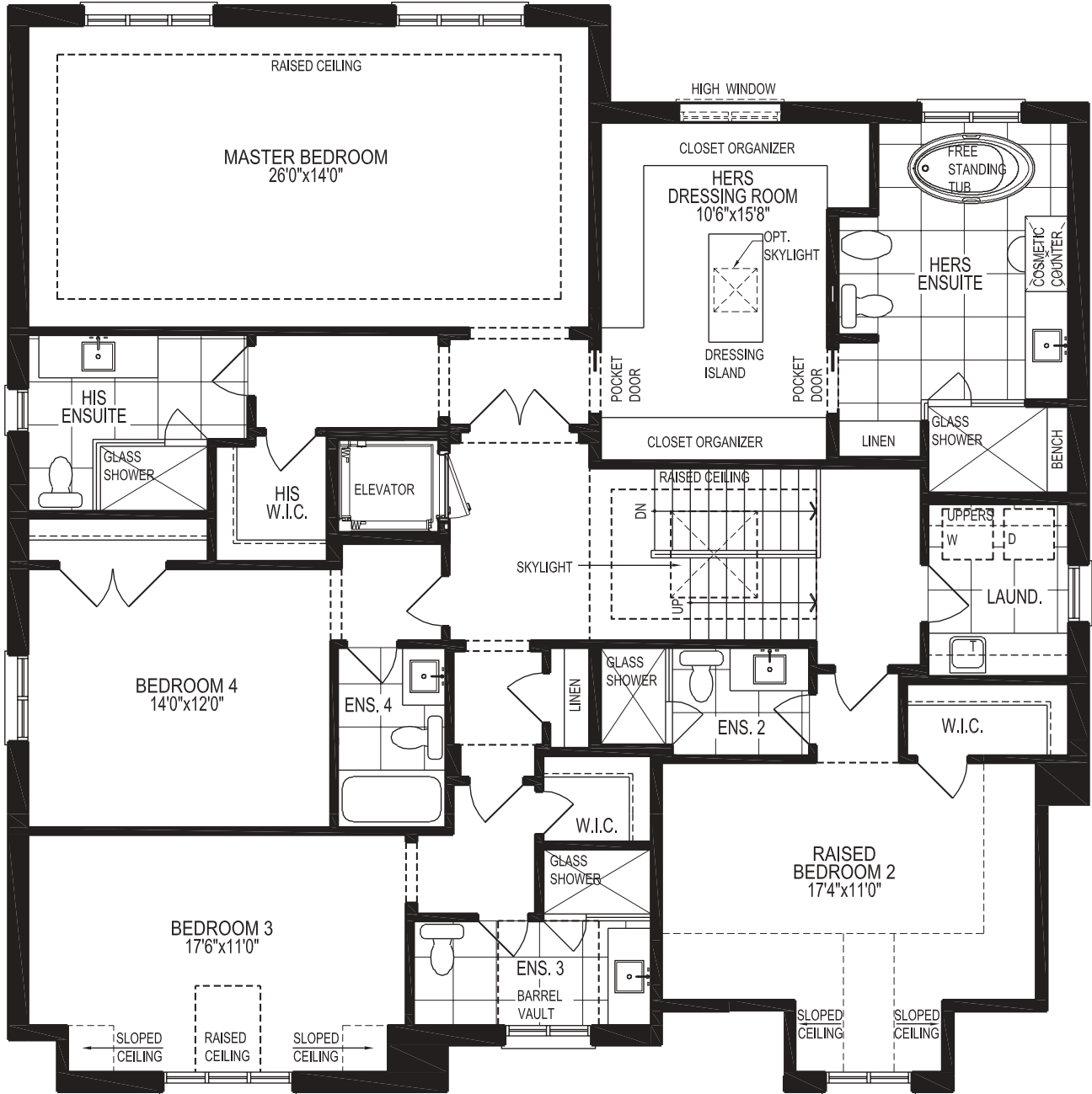
Elevation A SECOND FLOOR
