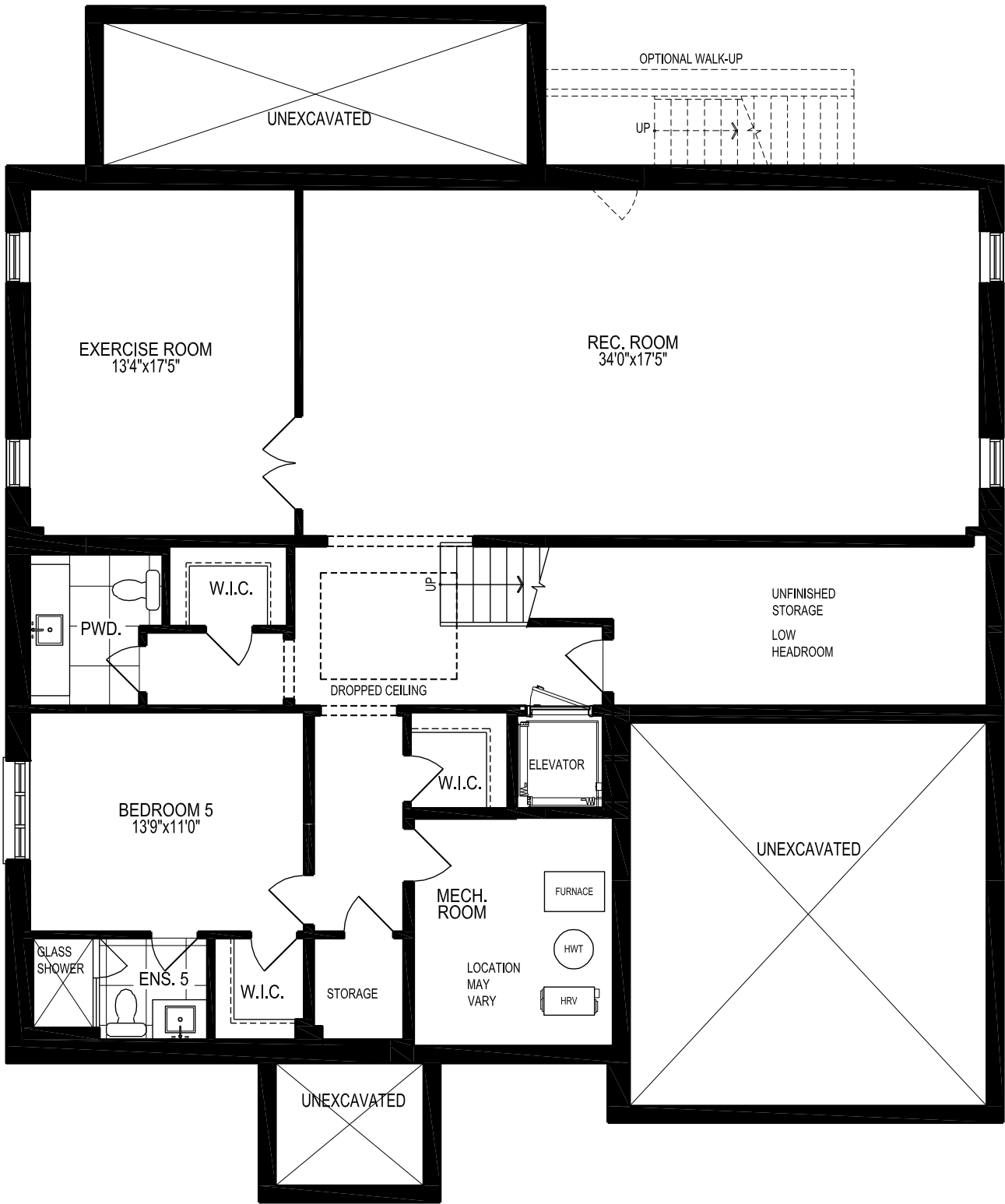
Elevation C BASEMENT
