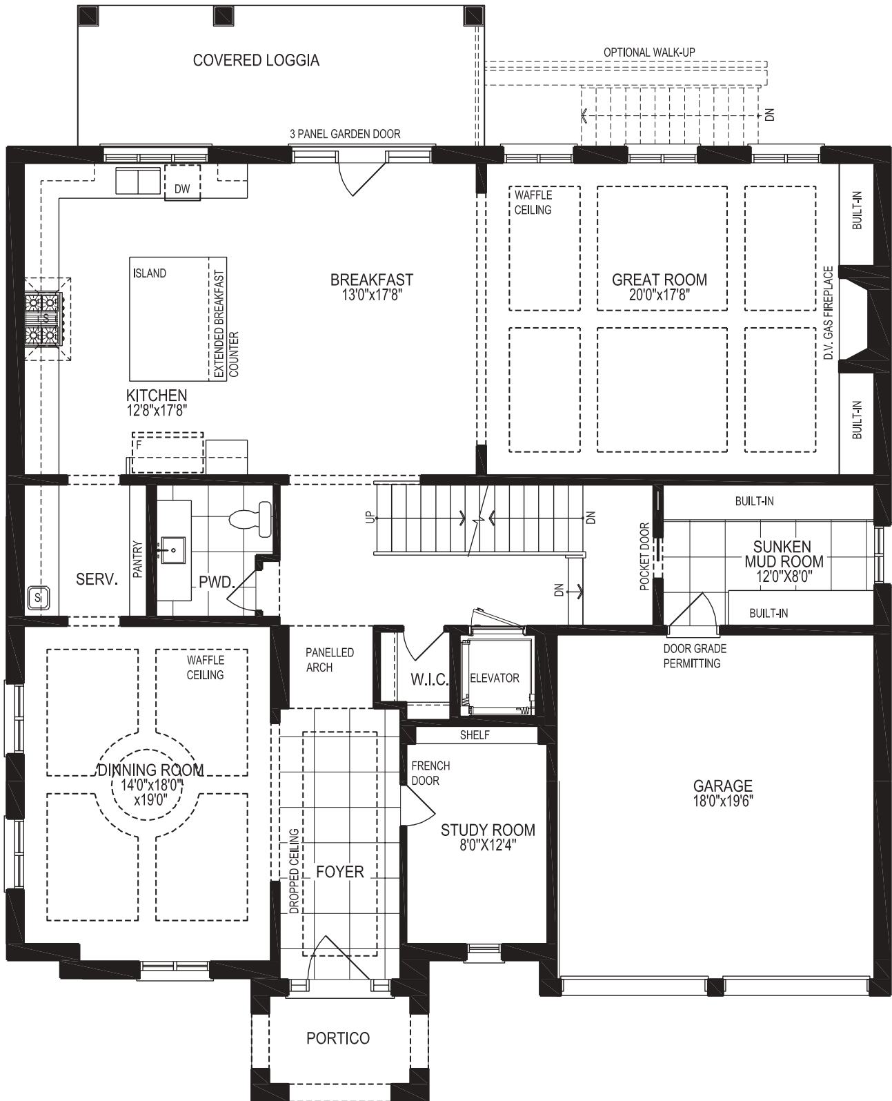
Elevation A GROUND FLOOR
