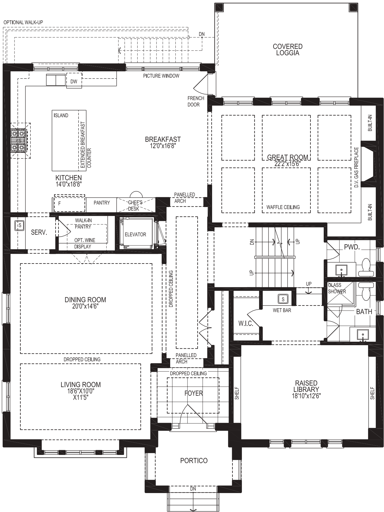
Elevation A GROUND FLOOR
