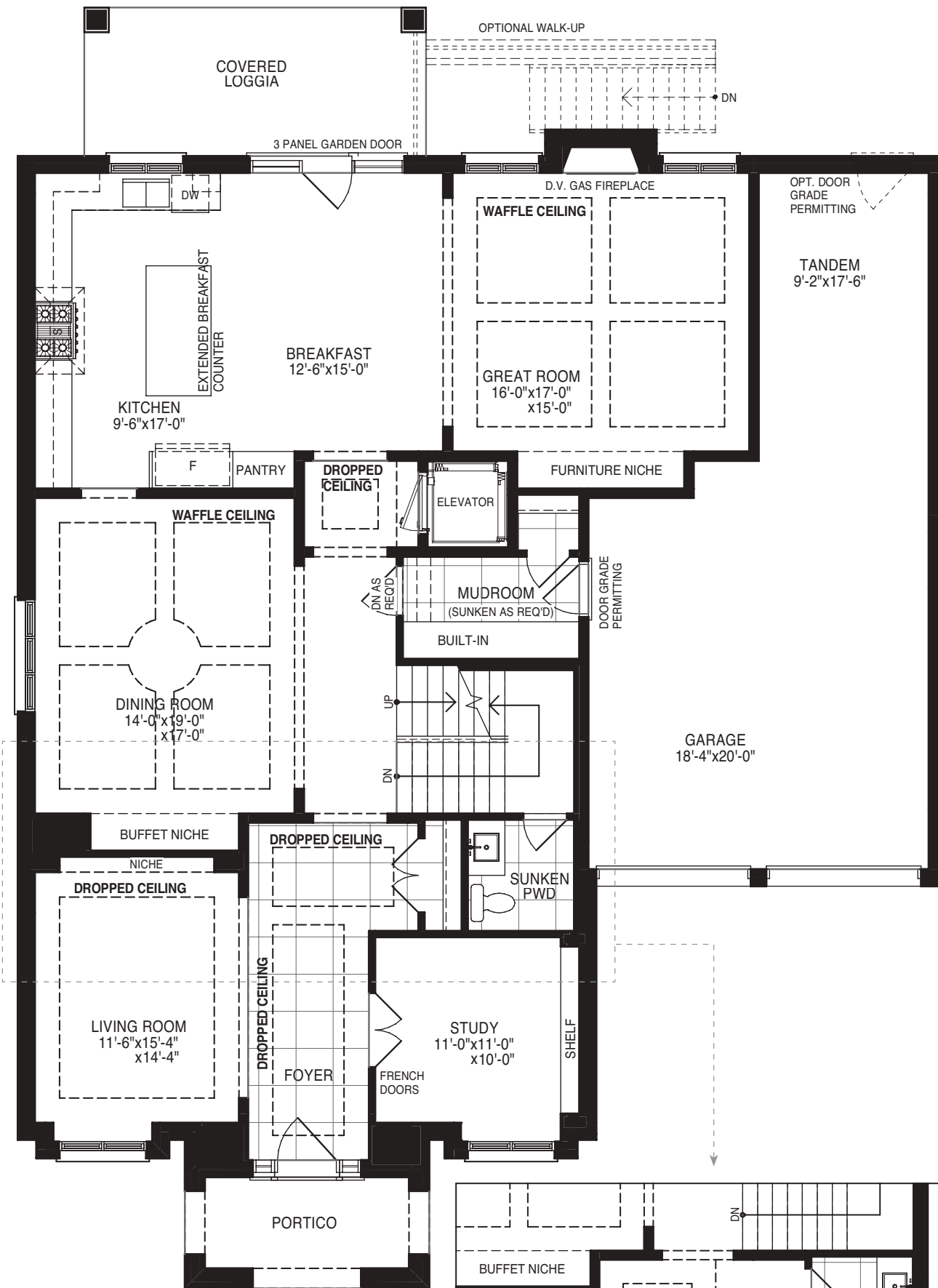
Elevation A GROUND FLOOR with tandem
