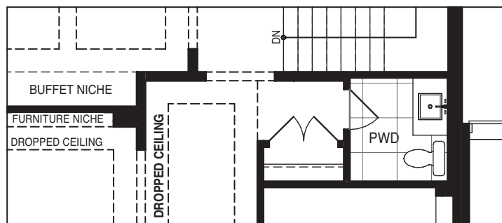
Elevation A OPT. PART. GROUND FLOOR W/O SUNKEN PWD
