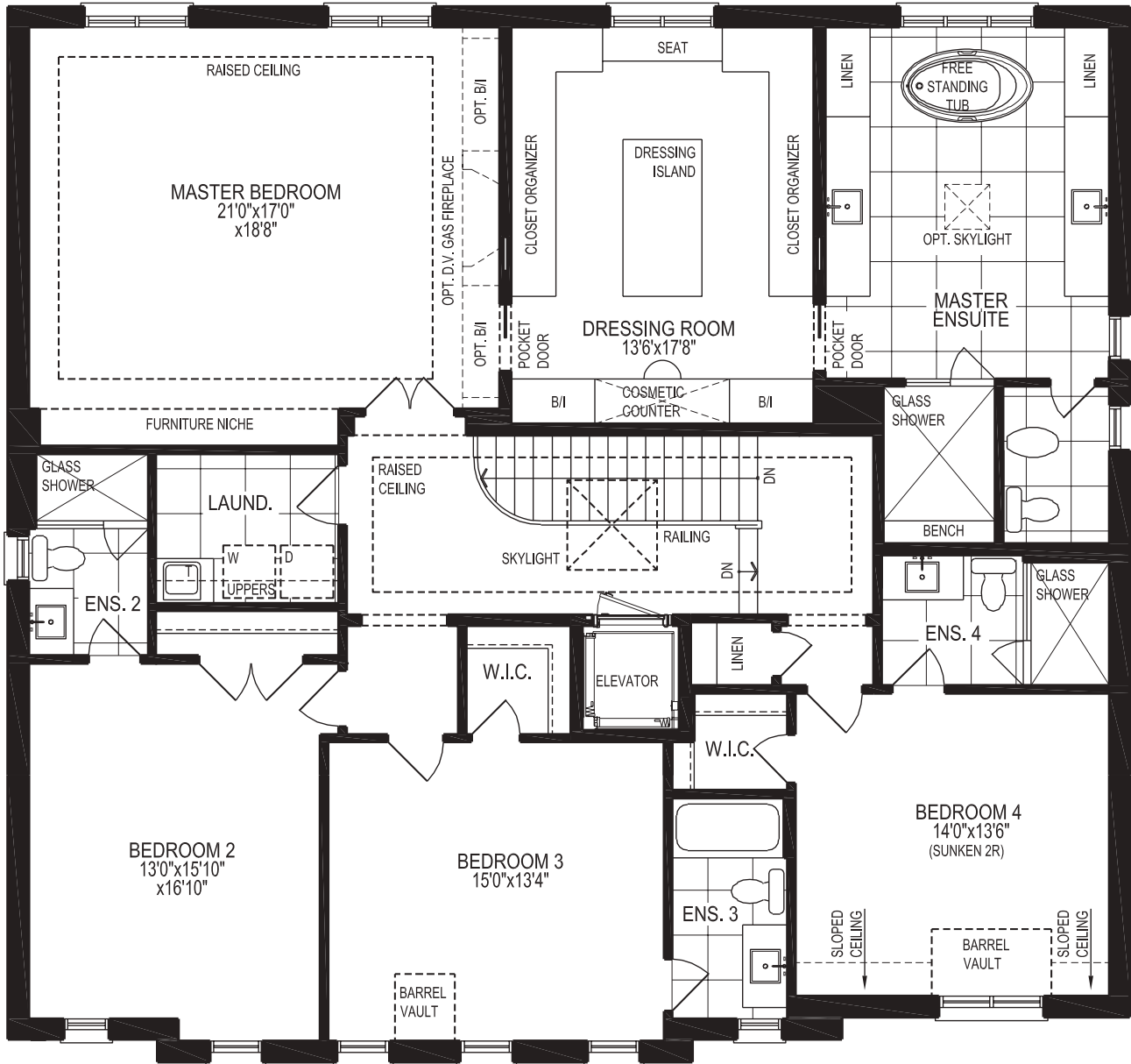
Elevation B SECOND FLOOR
