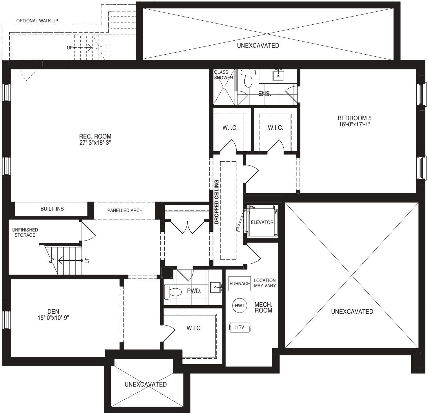
☆ ARCHITECT'S PREMIUM OPTION Elevation C BASEMENT
