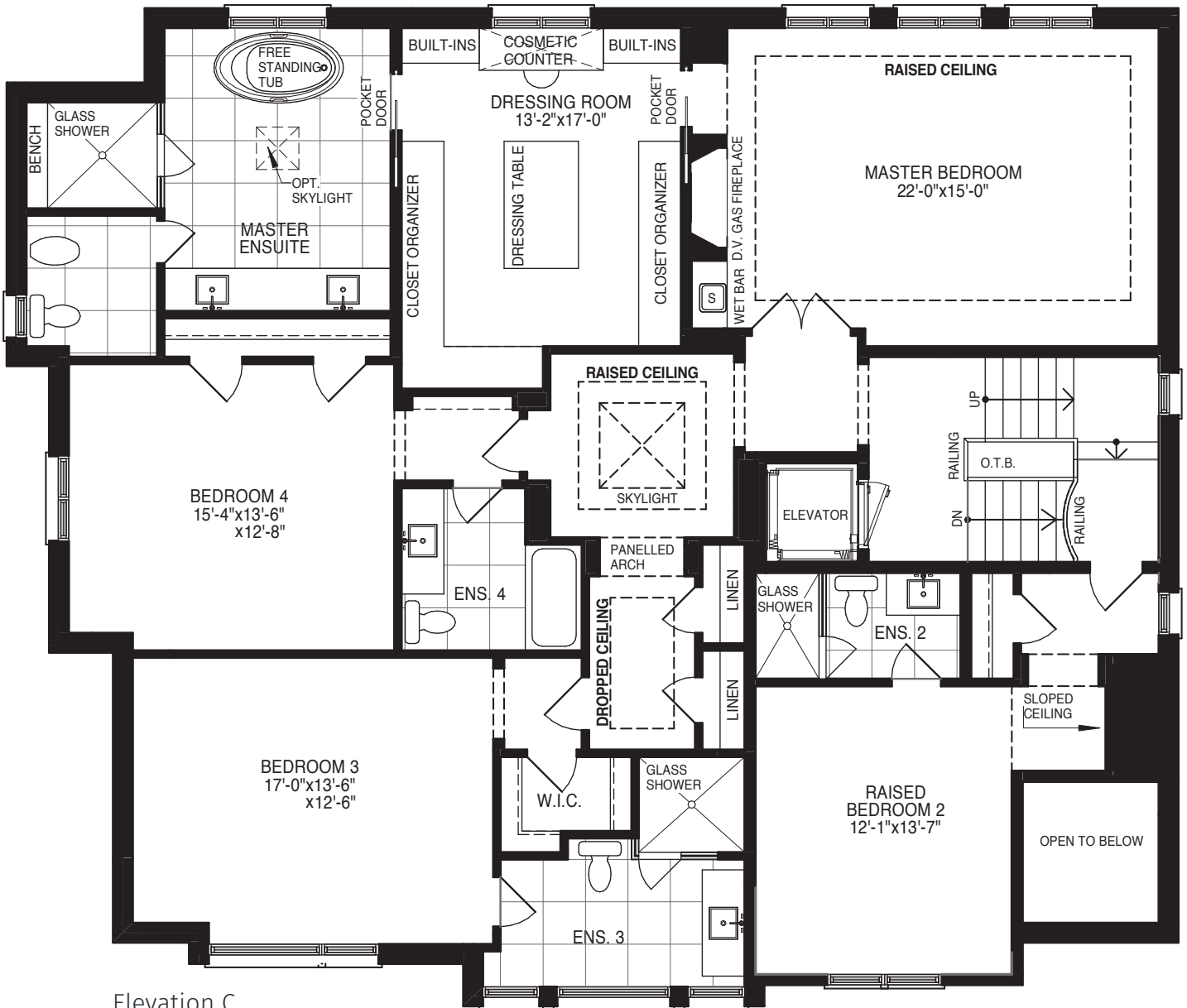
Elevation C SECOND FLOOR
