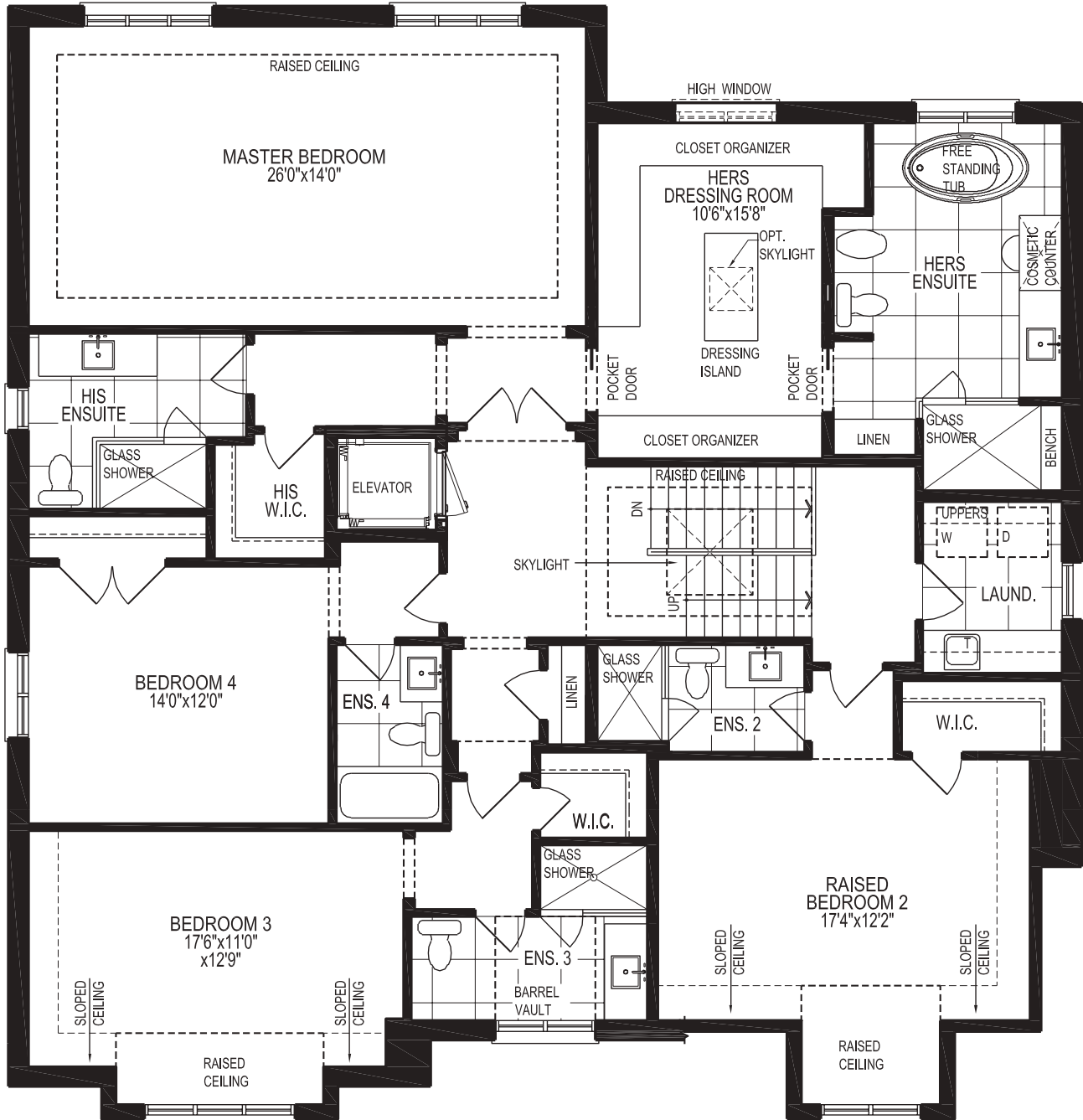
Elevation B SECOND FLOOR
