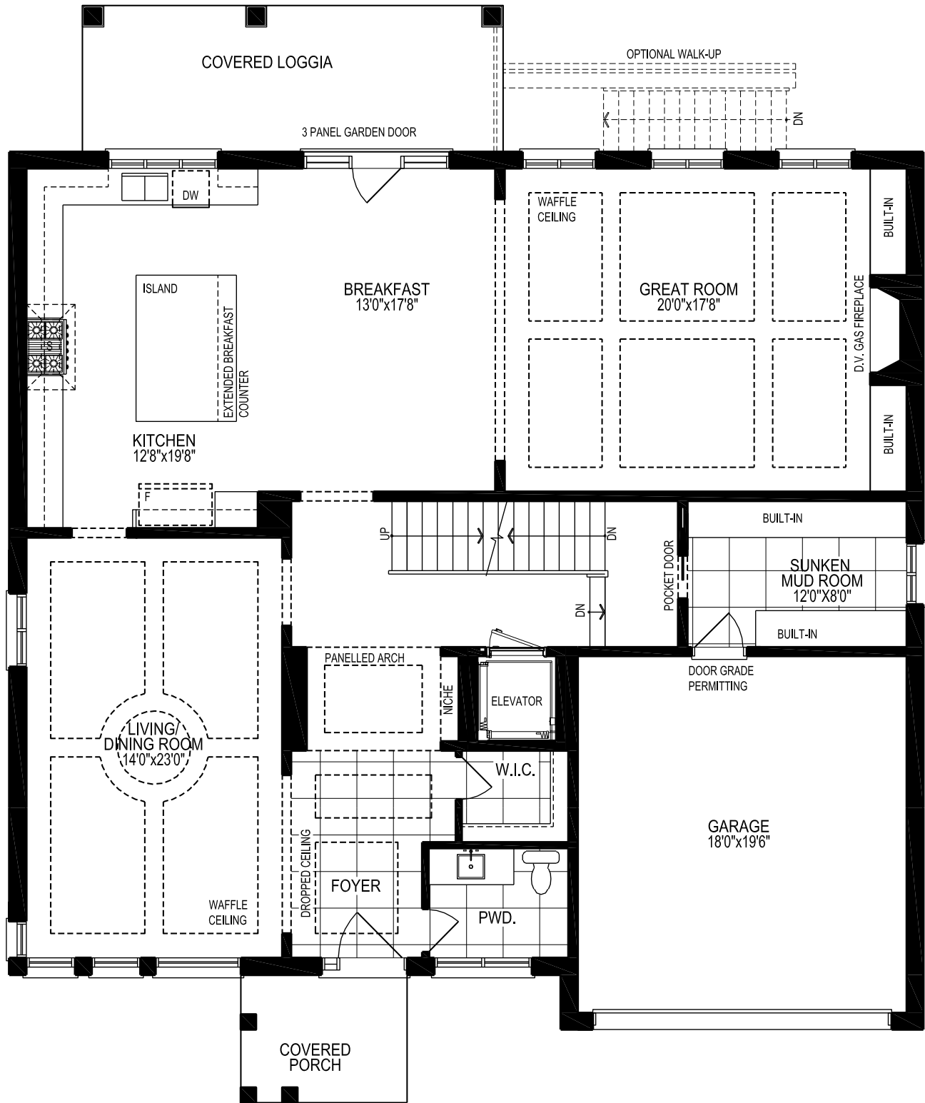
☆ ARCHITECT'S PREMIUM OPTION Elevation C GROUND FLOOR
