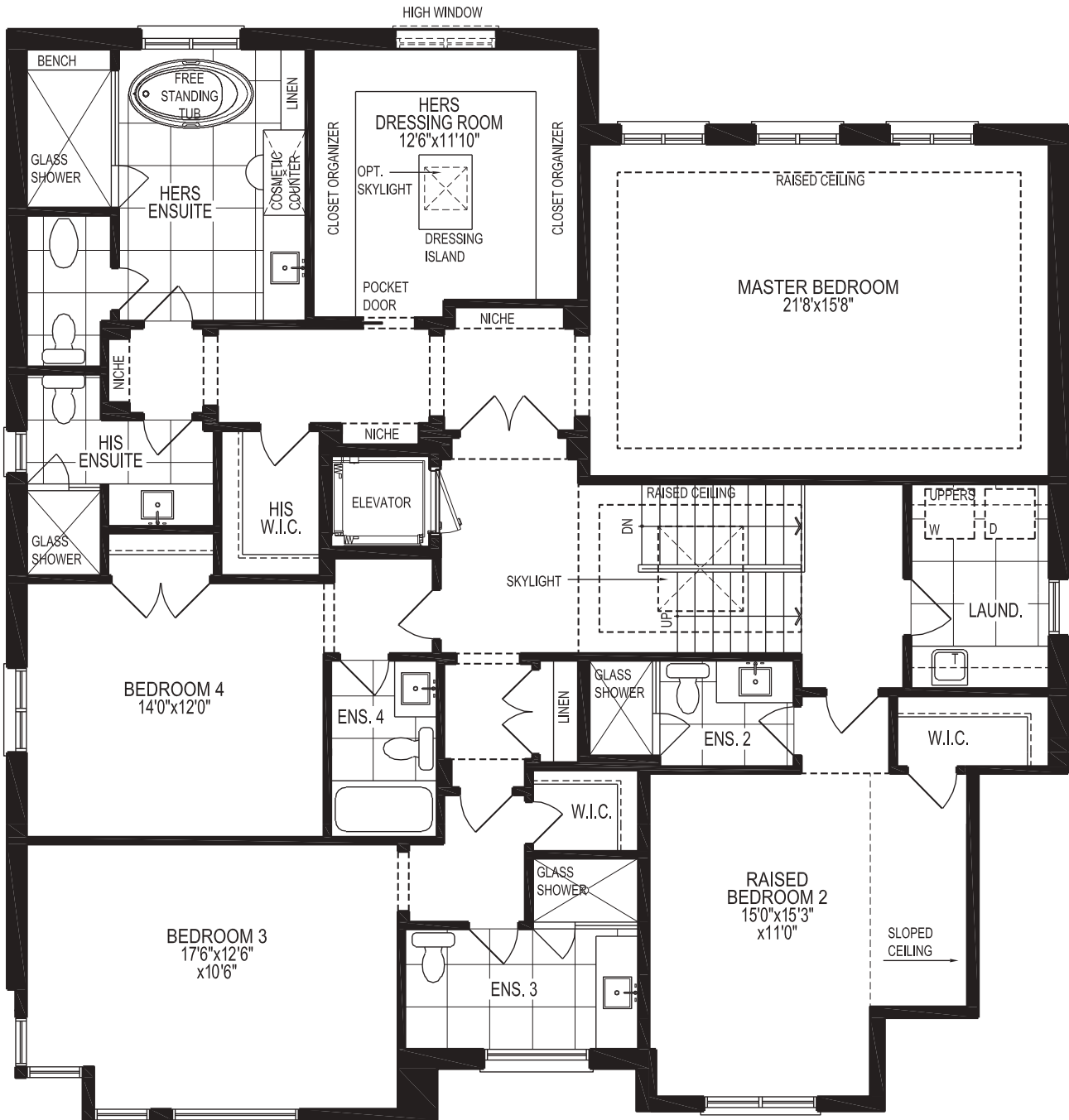
☆ ARCHITECT'S PREMIUM OPTION Elevation C SECOND FLOOR with his & her ensuite
